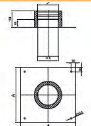
Base plate for chimney raise / DWECO - 08
