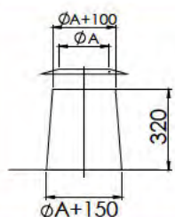
Steel Flat Flashing + Storm Collar / DWECO - 52
