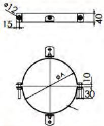
Swivel ring (ceiling hanger) / DWECO - 1062
