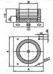
Base plate with condensate outlet at bottom / DWECO - 05
