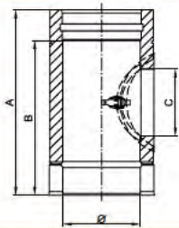
Inspection length with door 40 pa (N1) / DWECO - 68
