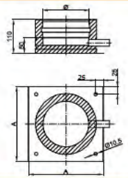
Base plate with side drain / DWECO - 66
