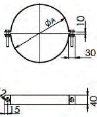
Split ring / DWECO - 1063
