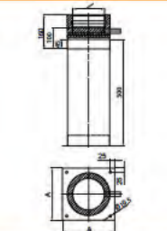
Adjustable base support 60 - 520 mm / DWECO - 03
