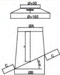
Flashing 16° - 25° lead base + Storm Collar / DWECO - 59
