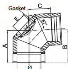
Elbow 87° with inspection / DWECO - 67
