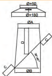
Flashing 36° - 45° lead base + Storm Collar / DWECO - 54
