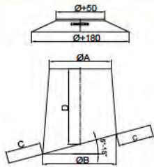
Flashing 5° - 15° lead base + Storm Collar / DWECO - 53
