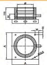
Base plate with lateral condensate outlet / DWECO - 06
